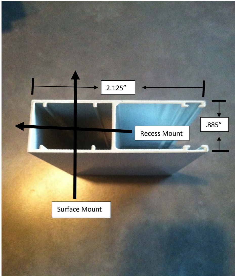
44mm Shutter Rail
